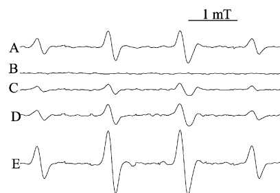
Fig. 6 Spectrum A, ESR spectrum of DMPO-hydroxyl radical adduct resulting from irradiation of an oxygen-saturated buffer solution of HBCD (0.4 mM, pH 7) and DMPO (50 mM). Spectrum B, in the absence of HBCD, oxygen or light. Spectrum C, similar to spectrum A, but in the presence of sodium benzoate (10 mM). Spectrum D, similar to spectrum A, but with HB instead of HBCD. Spectrum E, similar to spectrum A, but MAHB was used instead of HBCD. Spectral parameter settings: microwave power, 1.0 mW; time constant, 20.48 ms; modulation amplitude, 2.0 G; receiver gain, 1 \times 10^5 .
