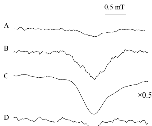
Fig. 3 Spectrum A, TR-ESR spectrum of argon-saturated HBCD (1 mM) DMSO–buffer solution (1:1 v/v, pH 7) measured 420 ns after the laser flash. Spectrum B, similar to spectrum A but in the presence of calf thymus DNA (2.85 mM). Spectrum C, similar to spectrum A but in the presence of aniline (2.85 mM). Spectrum D, similar to spectrum B, but with added methylene blue (1 mM). Spectral parameter settings: microwave power, 8.0 mW; time constant, 20.48 ms; modulation amplitude, 2.0 G; receiver gain, 1 \times 10^5 .
