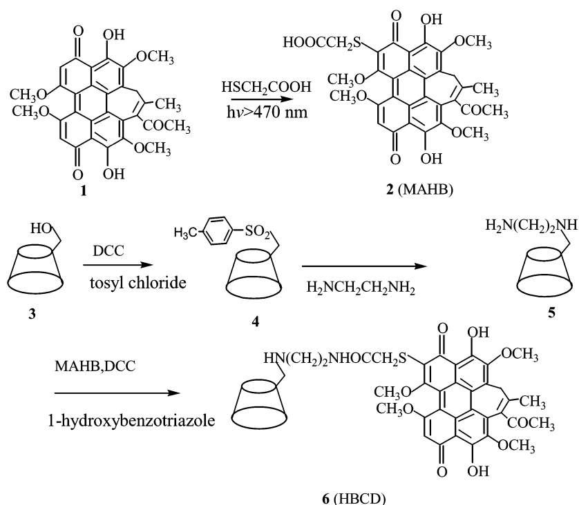
Scheme 1 Synthesis of cyclodextrin modified hypocrellin.
