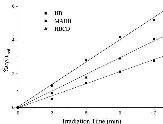
Fig. 5 Reduction of cytochrome c (58 \mu\text{M} ) in oxygen-saturated buffer solution (pH 7) by hypocrellins (10 \mu\text{M} ) as a function of irradiation time.
