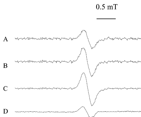
Fig. 2 Spectrum A, photoinduced ESR spectrum of a deaerated solution of HBCD (0.1 mM) in DMSO–buffer (1:1 v/v, pH 7), illuminated with 532 nm laser light for 15 min. Spectrum B, similar to spectrum A but in the presence of calf thymus DNA (2.85 mM). Spectrum C, similar to spectrum A, but in the presence of aniline (2.85 mM). Spectrum D, similar to spectrum B but with the addition of methylene blue (0.1 mM). Spectral parameter settings: X-band, microwave power, 8.0 mW; time constant, 20.48 ms; modulation amplitude, 2.0 G; receiver gain, 1 \times 10^5 .
