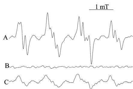
Fig. 4 Spectrum A, ESR spectrum of DMPO-superoxide radical adduct produced from irradiation of an oxygen-saturated DMSO solution of HBCD (0.2 mM) and DMPO (50 mM) for 2 min. Spectrum B, in the absence of HBCD, oxygen or light. Spectrum C, similar to spectrum A but in the presence of SOD ( 40 \mu\text{g ml}^{-1} ). Spectral parameter settings: microwave power, 1.0 mW; time constant, 20.48 ms; modulation amplitude, 1.0 G; receiver gain, 1 \times 10^5 .
