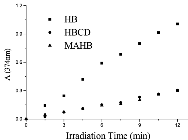
Fig. 8 DPA (0.6 mM) bleaching in oxygen-saturated DMSO photo-sensitized using hypocrellins ([HB] = 11.2 \mu\text{M} , [HBCD] = 10 \mu\text{M} , [MAHB] = 13.5 \mu\text{M} ) by measuring the absorbance decrease ( \Delta A ) at 374 nm for different irradiation times.
