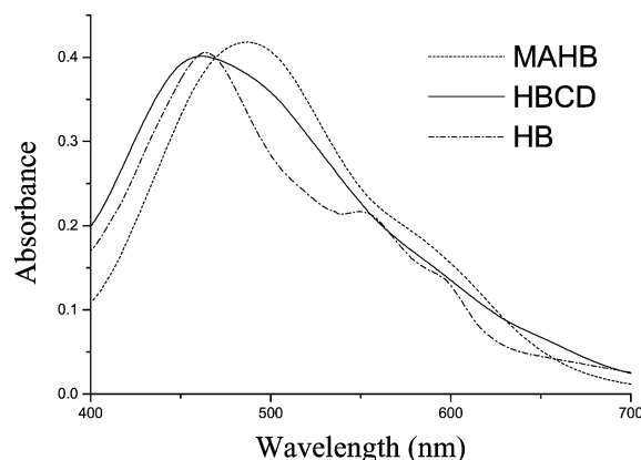
Fig. 1 Absorption spectra of HB, HBCD and MAHB in DMSO–buffer solution (1:1 v/v, pH 7).
